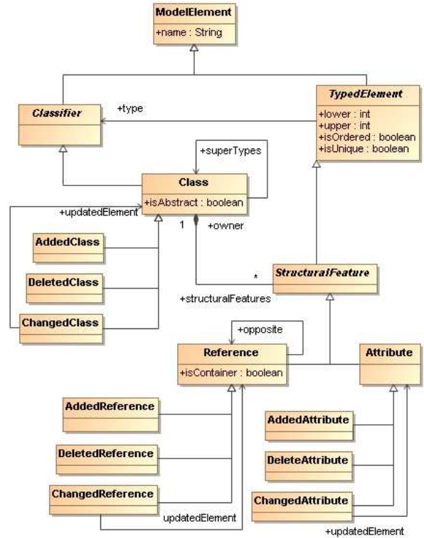
Figure 4. Generated difference KM3 meta-model
