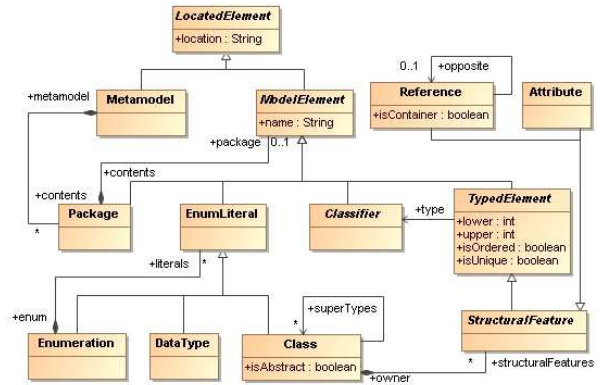
Figure 2. KM3 metamodel
