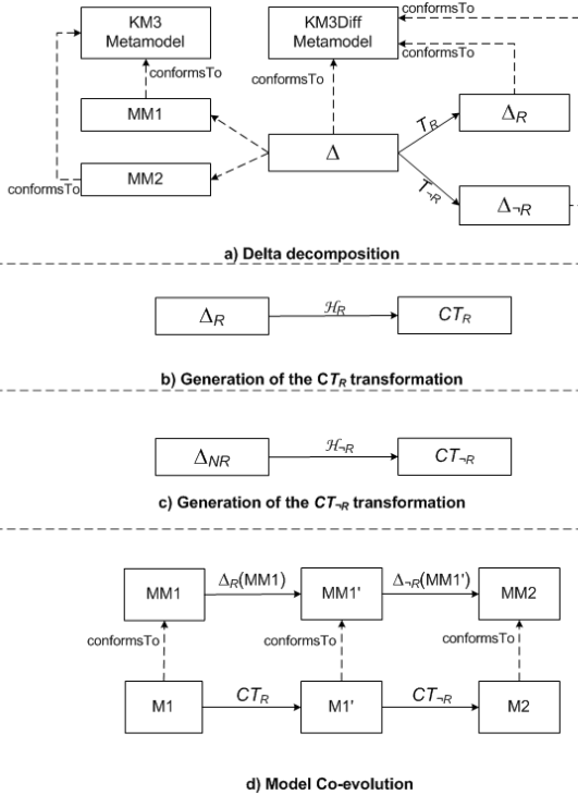
Figure 6. Overall approach
