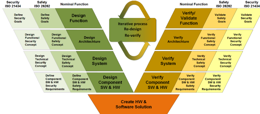
Fig. 3. Co-engineering of automotive Safety (ISO 26262) and Security (ISO/SAE 21434)
