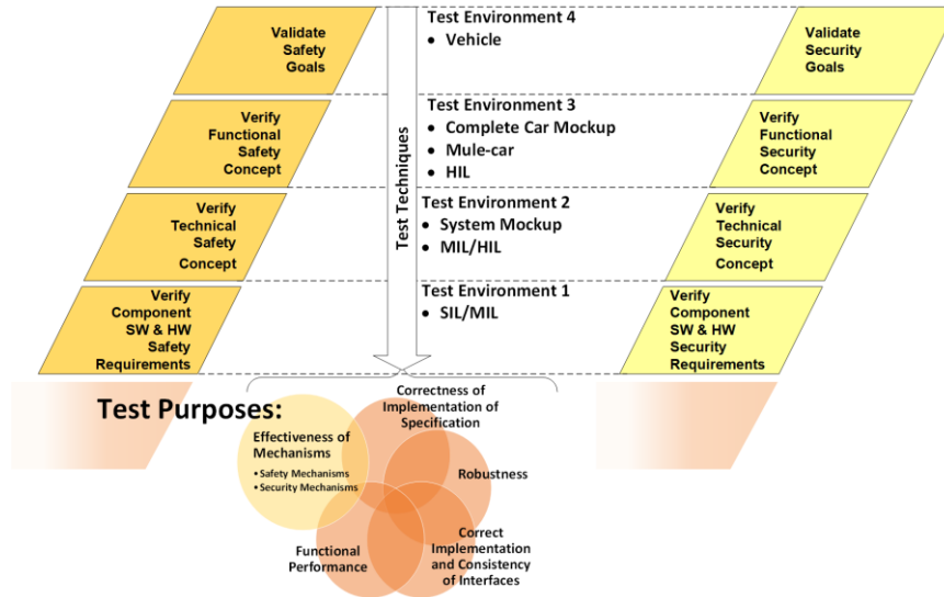
Fig. 4. Test techniques and test purposes at different integration levels and environments.
