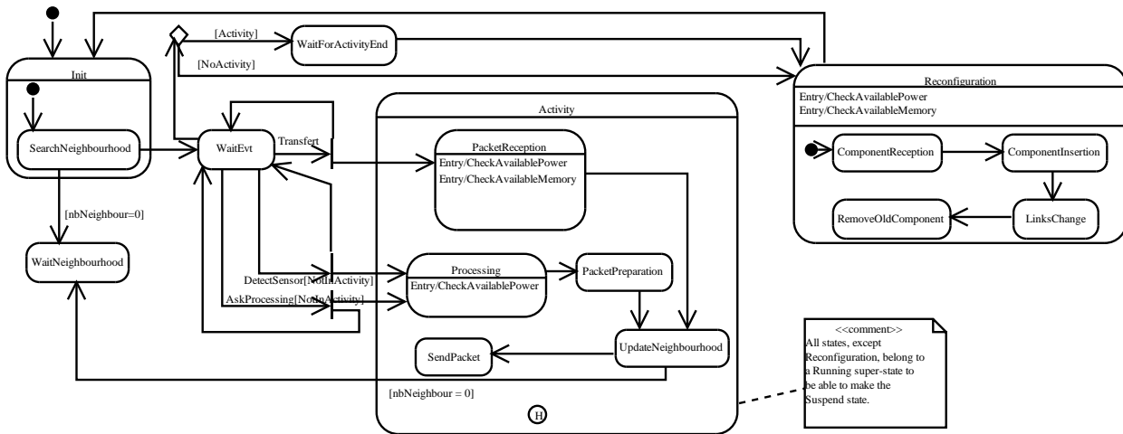
Fig. 2. The states of a sensor
