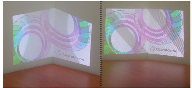
Figure 4. Left: A photograph of the visible key-distortion problem when the separation between the camera and the projector is high. Right: This photograph shows that there is no visible key-distortion effect when the camera is placed close to the pico projector, although the surface is curved.
